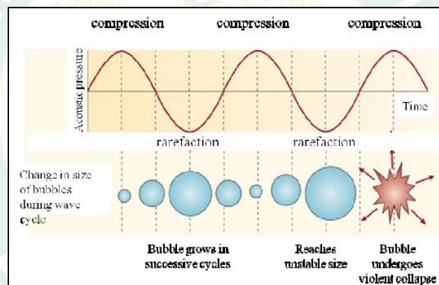
Figure 8 Cavitation phenomenon
