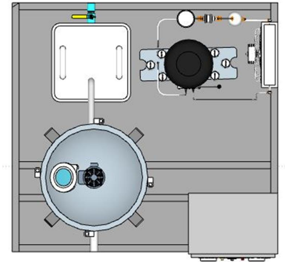
Figure 70 Assembly view of creamed honey maker (Top view)
