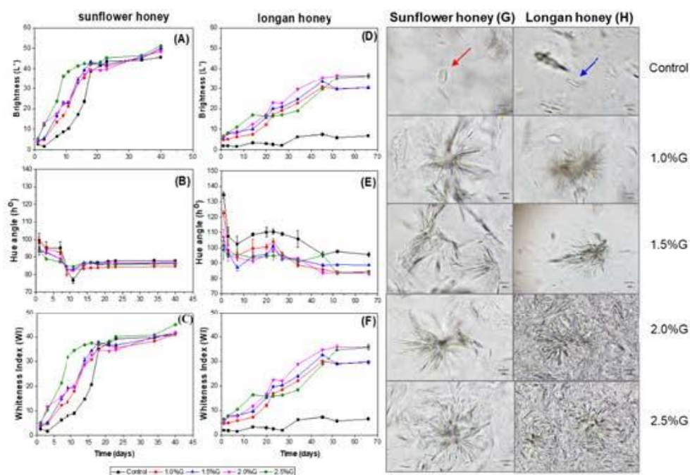
Figure 3. The L^* value, hue angle ( h^\circ ), and Whiteness Index (WI) of (A) - (C) sunflower honey and (D) - (F) longan honey in different amounts of glucose powder addition during storage; and microscopic observation of honey crystals at the end of crystallisation for (G) sunflower honey and (H) longan honey.
