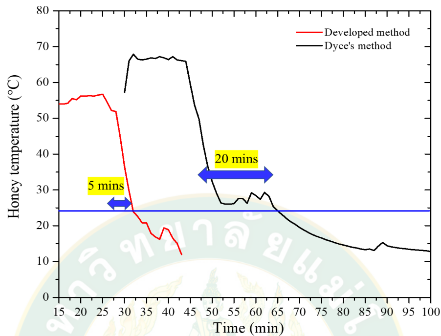
Figure 37 Honey temperature profile during rapid cooling rate at 6.50^{\circ}\text{C}/\text{min} comparing between Dyce's method and developed method
