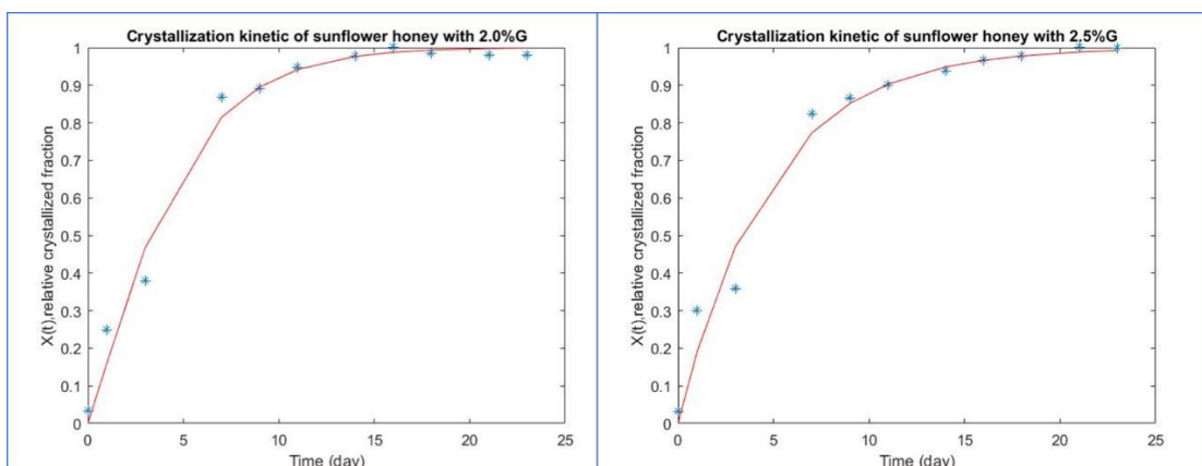
Figure 57 Nonlinear regression for crystallization kinetic from Avrami equation by MATLAB program (sunflower honey)
