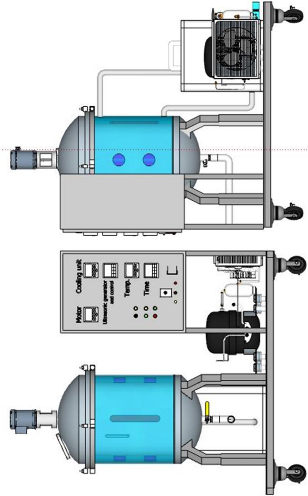
Figure 68 Assembly view of creamed honey maker (side view-1)
