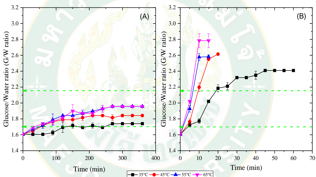
Figure 19 G/W ratio variation with dehydration time of longan honey by (A) Hot air oven (B) Vacuum far-infrared dryer at different temperature
